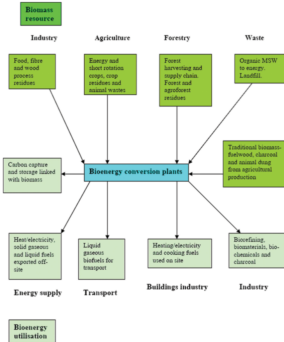
Figure 4: Biomass resources from several sources are converted into a range of products for use by transport, industry, and building sectors. [27]
