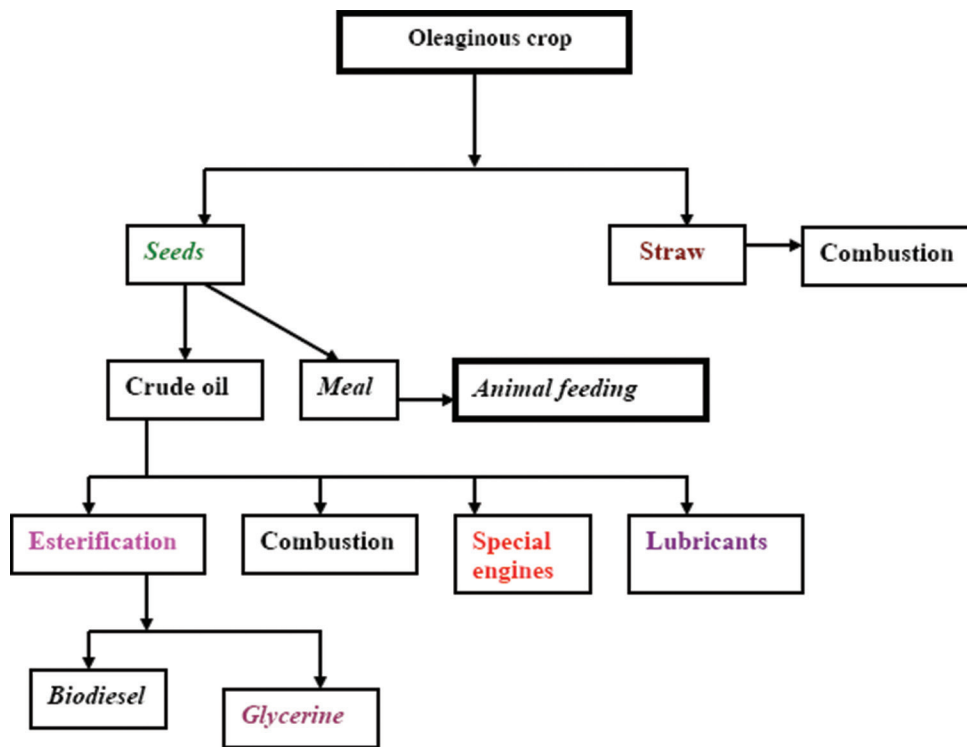
Figure 9: Flow chart of biodiesel production [32]
