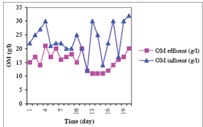
Figure 5: Organic matters before and after treatment in digester [29]
