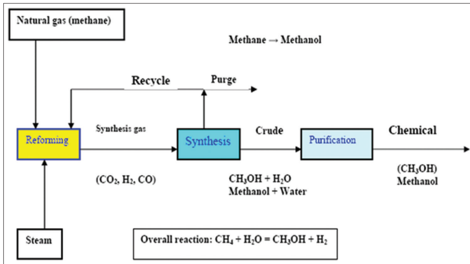
Figure 2: Schematic diagram shows methanol production [16]
